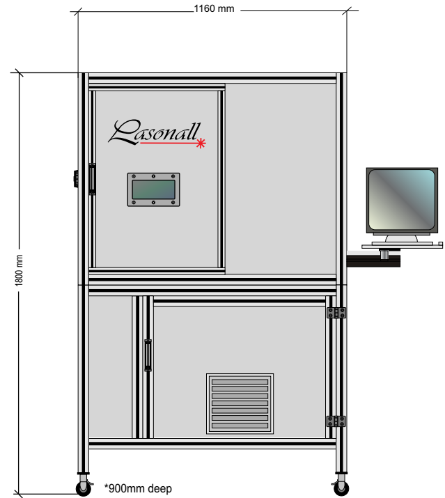
Part Loading Door-Face View
